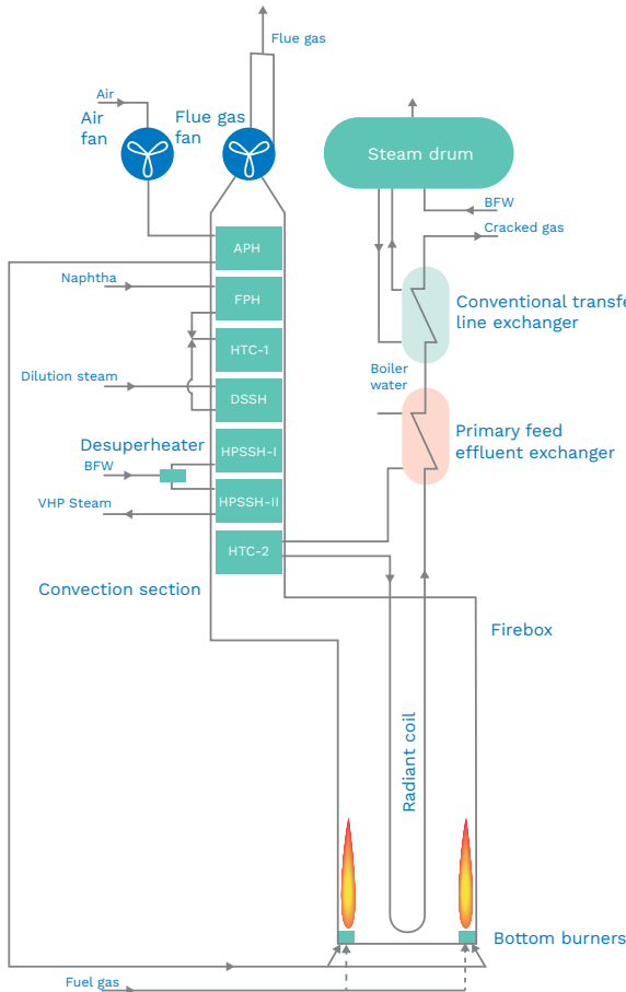
Low-emission cracking furnace with air preheat and boiler coil.
