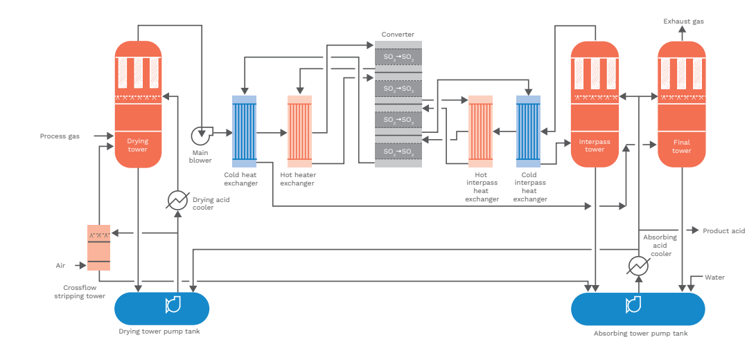
Typical MECS® metallurgical plant flowsheet:
