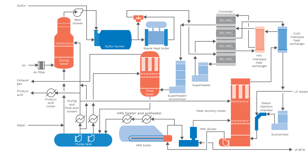
Typical MECS® sulfur burning plant flowsheet, including HRS™ system:
