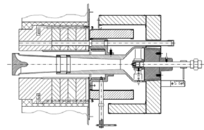
TSWB® drawing
